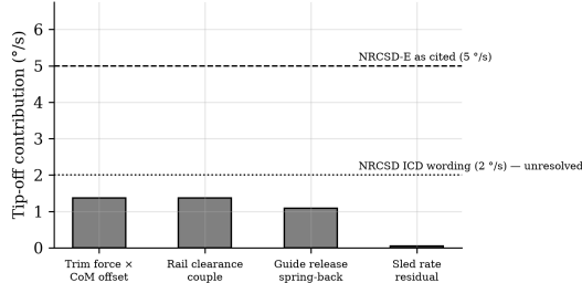
Fig. 11. Tip-off error budget against deployer requirement classes.
