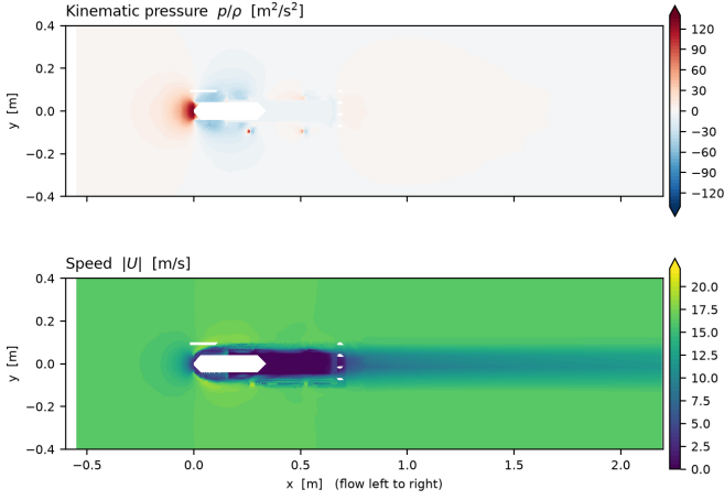
Fig. 17. Mid-plane slice ( z = 0 ) of the converged fine-mesh solution: kinematic pressure above, speed below, flow left to right. Stagnation on the forward face, separation at the shoulders, and a wake that has not recovered by x = 2.2 m. The pressure term shown here is integrated directly from the solved field; the viscous term is not solved and is bounded by a turbulent flat-plate correlation over the meshed wetted area, as the text states.
