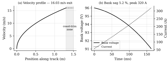
Fig. 9. Historical periodic-model shot profile: (a) velocity with coast-trim zone; (b) bank voltage and current.
