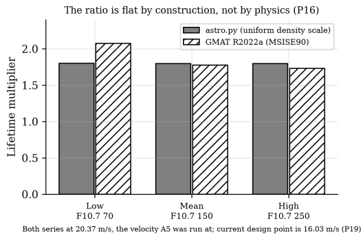
Fig. 13. Solar-activity sweep against GMAT. The static-atmosphere model returns a flat ratio by construction, not by physics; an independent propagator does not.
