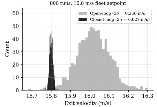
Fig. 9. Closed-loop exit-velocity dispersion, 800 Monte Carlo runs.
