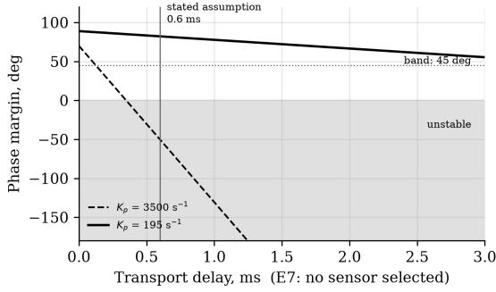
Fig. 7. Phase margin against transport delay. The earlier gain crosses into instability at 0.35 ms of transport delay; the designed gain holds more than 55^\circ across the whole swept range.
