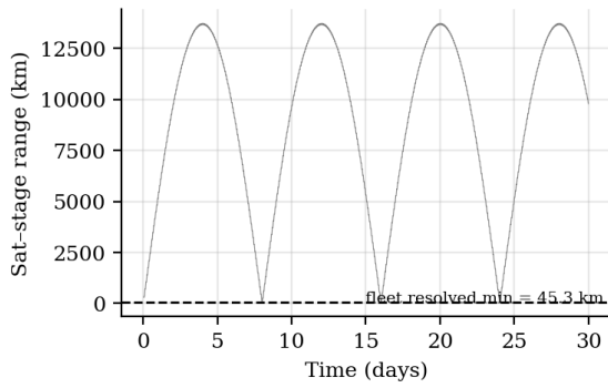
Fig. 10. Satellite-stage range over 30 days, staggered firing at the rated velocity.
