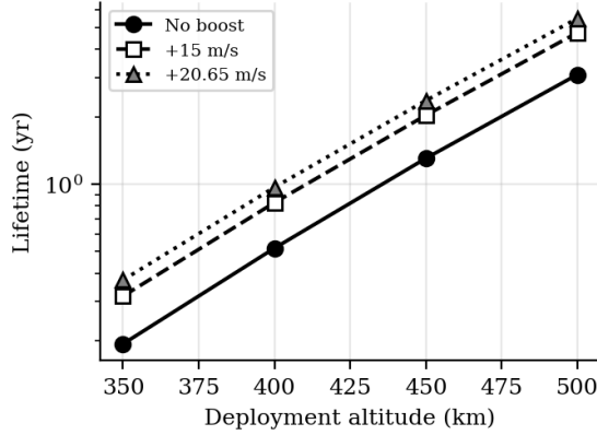
Fig. 7. Orbital lifetime vs deployment altitude ( BC = 61 \text{ kg/m}^2 , mean activity).
