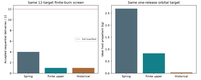
Fig. 22. Matched reference inputs and bounded optimizer outcomes. No sampled twelve-shot option closes; assumed device masses and host performance are not supplier data.
