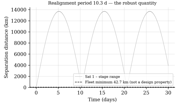
Fig. 14. Satellite-stage range over 30 days, staggered firing at the rated velocity.
