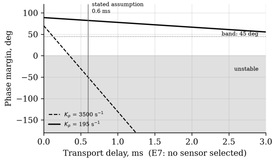
Fig. 7. Phase margin against transport delay. The earlier gain crosses into instability at 0.35 ms of transport delay; the designed gain holds more than 55° across the whole swept range.
