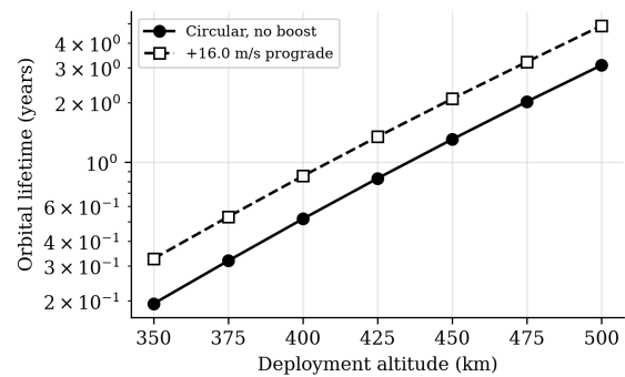
Fig. 11. Orbital lifetime vs deployment altitude (BC = 61 \text{ kg/m}^2 , mean activity).
