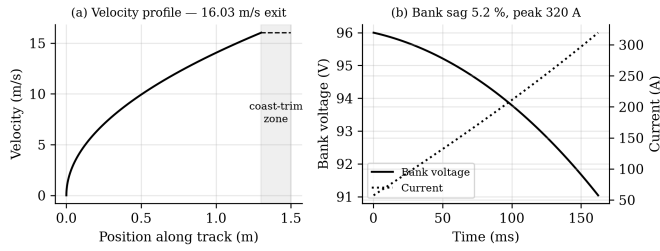
Fig. 8. Shot profile at the rated point: (a) velocity with coast-trim zone; (b) bank voltage and current.
