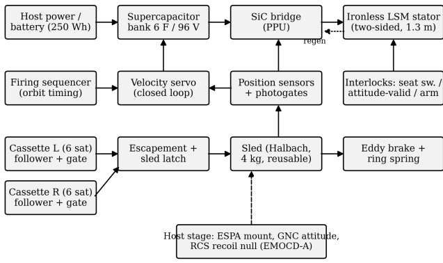
Fig. 1. System block diagram: power, control, mechanism, and host-interface chains.
