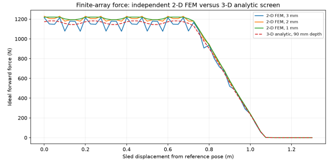
Fig. 21. Finite Gen5 force profiles from a 2-D magnetostatic FEM at three mesh sizes and the 3-D analytic cuboid-field screen. Both use ideal phase. The 2-D solve omits magnet-depth effects; no curve is a measurement.
