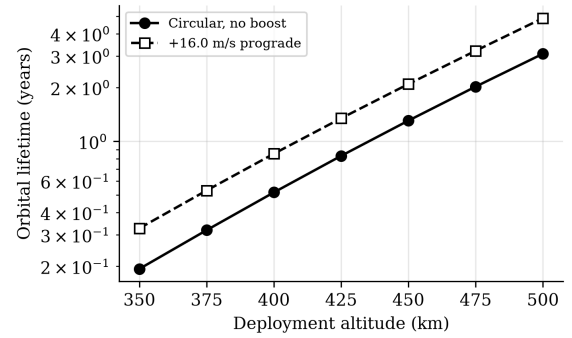
Fig. 11. Orbital lifetime vs deployment altitude (BC = 61 kg/m 2 , mean activity).
