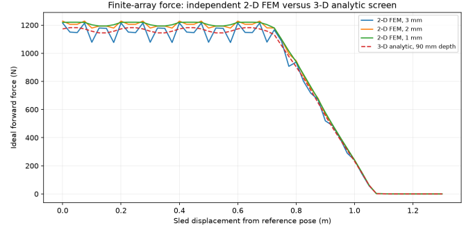
Fig. 22. Finite Gen5 force profiles from a 2-D magnetostatic FEM at three mesh sizes and the 3-D analytic cuboid-field screen. Both use ideal phase. The 2-D solve omits magnet-depth effects; no curve is a measurement.
