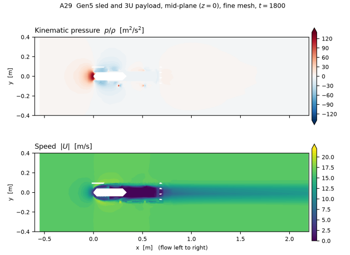
Fig. 18. Mid-plane slice ( z = 0 ) of the converged fine-mesh solution: kinematic pressure above, speed below, flow left to right. Stagnation on the forward face, separation at the shoulders, and a wake that has not recovered by x = 2.2 m. The pressure term shown here is integrated directly from the solved field; the viscous term is not solved and is bounded by a turbulent flat-plate correlation over the meshed wetted area, as the text states.
