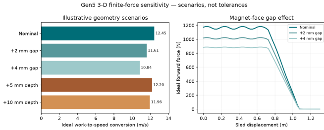
Fig. 23. Deterministic ideal-force scenarios for face gap and depth offset. The 14 mm face gap gives 0.907 kJ versus 1.042 kJ at 12 mm; these are assumed geometry changes, not measured tolerances or achieved speed.
