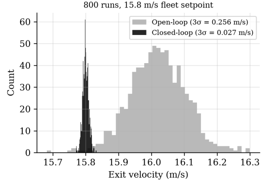
Fig. 10. Closed-loop exit-velocity dispersion, 800 Monte Carlo runs.
