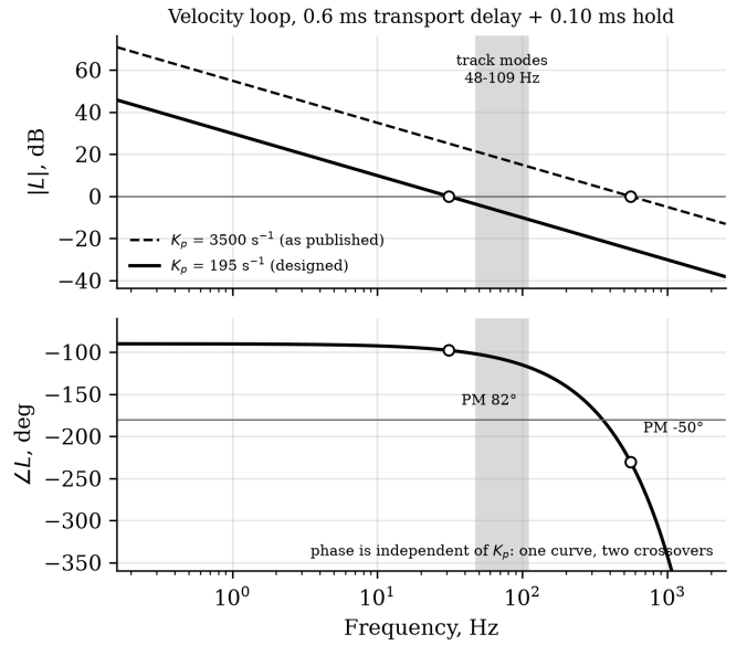
Fig. 7. Open-loop velocity-loop response at the earlier and the designed gain, with the 48–109 Hz band of track modes shaded and both gain crossovers marked. Phase depends only on frequency and delay, so the two gains share one phase curve.
