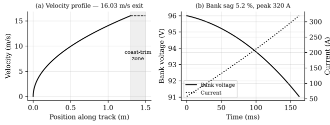
Fig. 9. Historical periodic-model shot profile: (a) velocity with coast-trim zone; (b) bank voltage and current.
