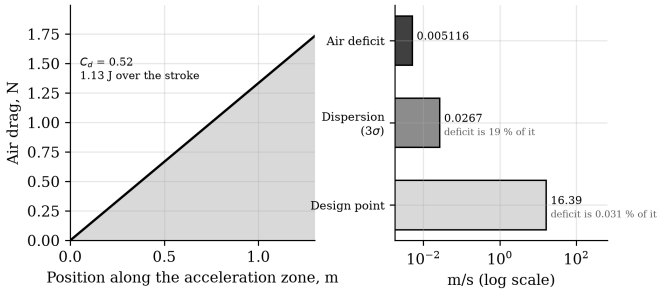
Fig. 20. Air drag along the acceleration zone, and the resulting exit-velocity deficit set against the design point and against the dispersion a ground test exists to resolve.
