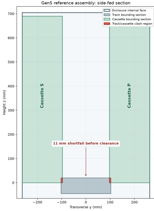
Fig. 21. Gen5 side-fed reference-section failure. The two cassette widths and track require 537 mm within a 526 mm internal width before clearance. FreeCAD and CadQuery exact-solid intersections each find 32,915 mm 3 overlap per side. A new feed or enclosure configuration would require renewed analysis.
