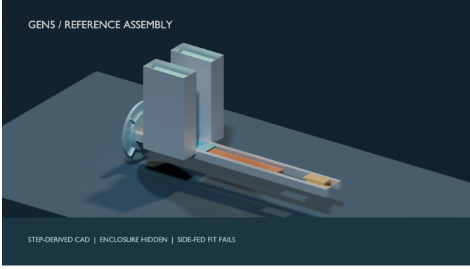
Fig. 3. Twenty-instance Gen5 reference assembly visualized in Blender after FreeCAD read-back of named STEP solids. The enclosure is hidden to expose the track and side cassettes. Their evaluated placement has a documented exact-solid interference; the image is geometry visualization, not a built or qualified mechanism.
