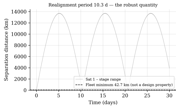
Fig. 15. Satellite-stage range over 30 days, staggered firing at the rated velocity.
