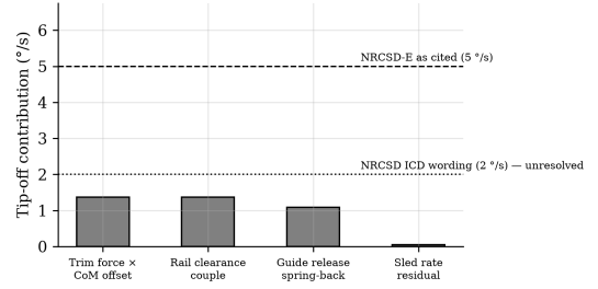
Fig. 16. Tip-off error budget against deployer requirement classes.
