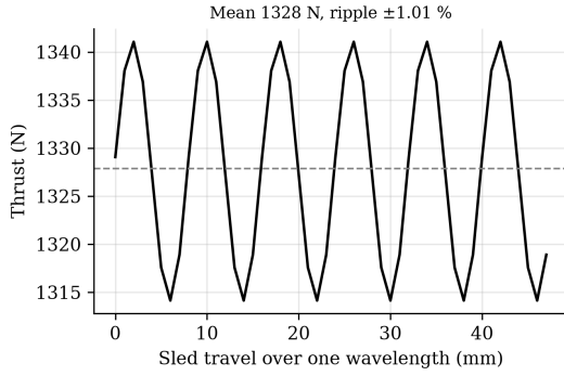
Fig. 6. Winding-resolved thrust over one wavelength of sled travel.
