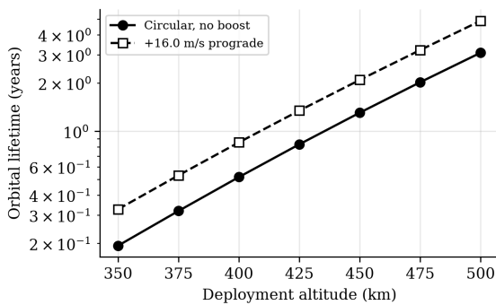
Fig. 12. Orbital lifetime vs deployment altitude (BC = 61 kg/m 2 , mean activity).
