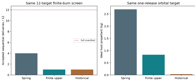
Fig. 22. Matched reference inputs and bounded optimizer outcomes. No sampled twelve-shot option closes; assumed device masses and host performance are not supplier data.
