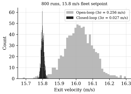
Fig. 9. Closed-loop exit-velocity dispersion, 800 Monte Carlo runs.
