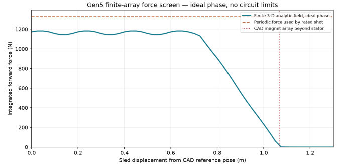
Fig. 21. Finite Gen5 analytic force map with ideal phase, contrasted with the historical periodic-force assumption. The curve is a model screen, not a FEM result or physical measurement.
