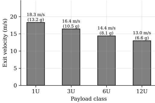
Fig. 12. Payload family: force-limited above 1U; velocity, not safety, is traded. † Counts are volumetric , calibrated so the 3U case returns the twelve the machine is laid out for. A subsequent fixed-cell design study replaces them where a cell geometry actually exists: 1U gives 36 per load at 2.125 kg , not 40 at 1.92, because three 100 mm units plus two dividers leave 37.5 mm of a 340.5 mm cell unusable, and ThinSat and 12U are refused outright because two of their dimensions exceed the 100 mm cell section. The binding constraint is the 166 mm cassette width.
