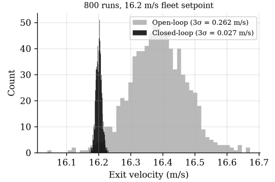
Fig. 6. Closed-loop exit-velocity dispersion, 800 Monte Carlo runs.
