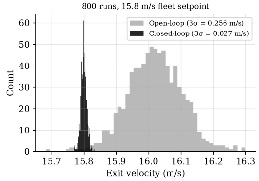
Fig. 10. Closed-loop exit-velocity dispersion, 800 Monte Carlo runs.
