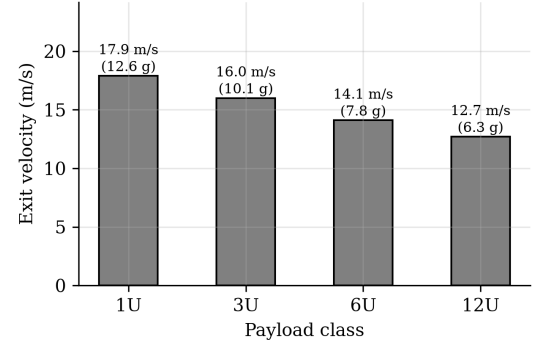
Fig. 17. Payload family: force-limited above 1U; velocity, not safety, is traded. †Counts are volumetric, calibrated so the 3U case returns the twelve the machine is laid out for. A subsequent fixed-cell design study replaces them where a cell geometry actually exists: 1U gives 36 per load at 2.125 kg , not 40 at 1.92, because three 100 mm units plus two dividers leave 37.5 mm of a 340.5 mm cell unusable, and ThinSat and 12U are refused outright because two of their dimensions exceed the 100 mm cell section. The binding constraint is the 166 mm cassette width.
