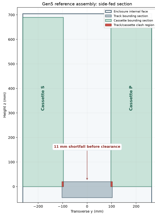
Fig. 21. Gen5 side-fed reference-section failure. The two cassette widths and track require 537 mm within a 526 mm internal width before clearance. FreeCAD and CadQuery exact-solid intersections each find 32,915 mm 3 overlap per side. A new feed or enclosure configuration would require renewed analysis.
