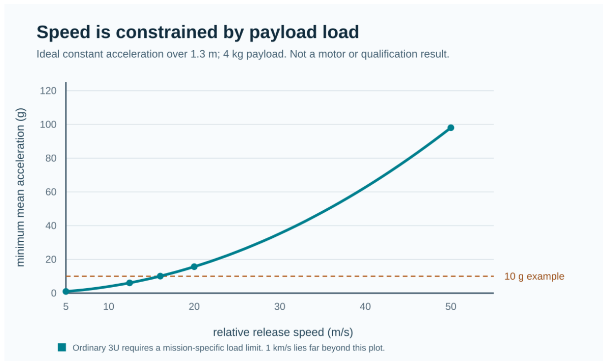
Figure 8: Ideal acceleration required by speed on a 1.3 m stroke; not a VOLLEY motor rating.
