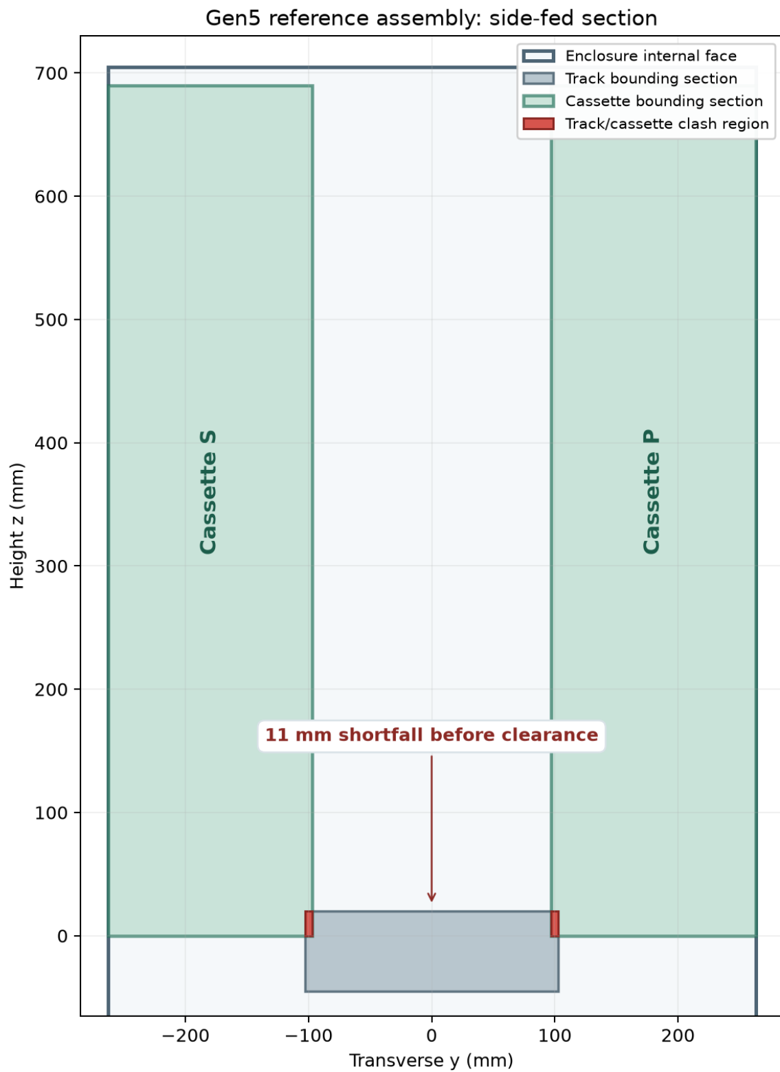
Figure 16: Dimensioned side-fed reference cross-section; this configuration fails the width check.
