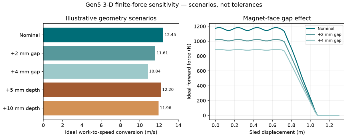
Figure 4: Ideal gap/depth sensitivity; scenarios rather than measured tolerances.
