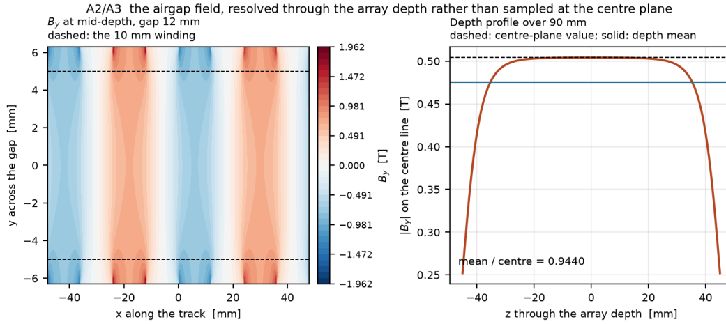
Figure 11: Representative magnetic-field model output. Source: thesis figure A02.
