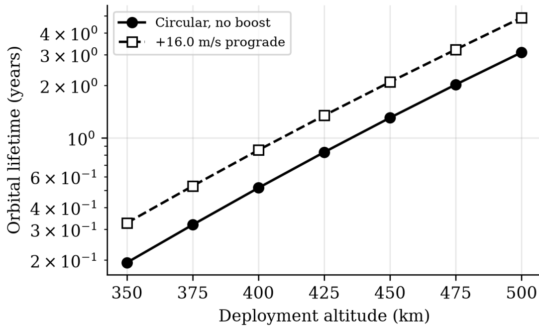
Figure 14: Modelled orbital-lifetime response. Absolute values depend on atmosphere.
