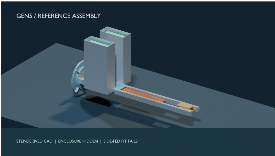
Figure 1: Gen5 reference FreeCAD/STEP assembly visualized in Blender with enclosure hidden. Known side-fed clash remains; no physical article exists.
