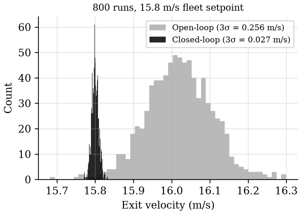
Figure 12: Closed-loop simulation distribution at the fleet setpoint.
