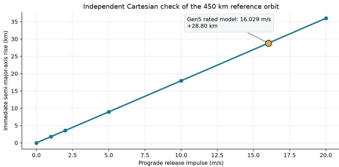
Figure 13: Independent rated-state two-body orbit check. The lifetime claim is outside its scope.
