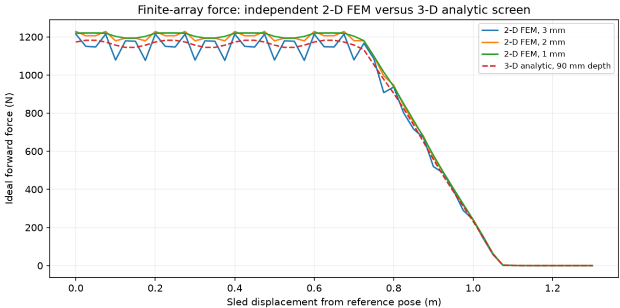
Figure 3: Independent 2-D finite-element force screen, not a measurement.
