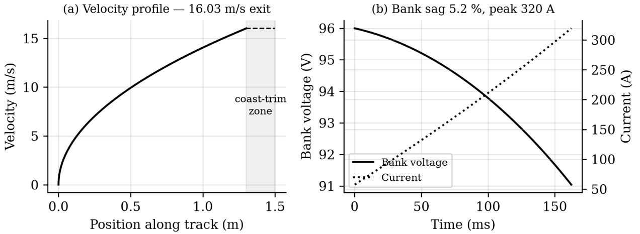
Figure 10: Historical modeled shot: velocity, bank voltage and current.
