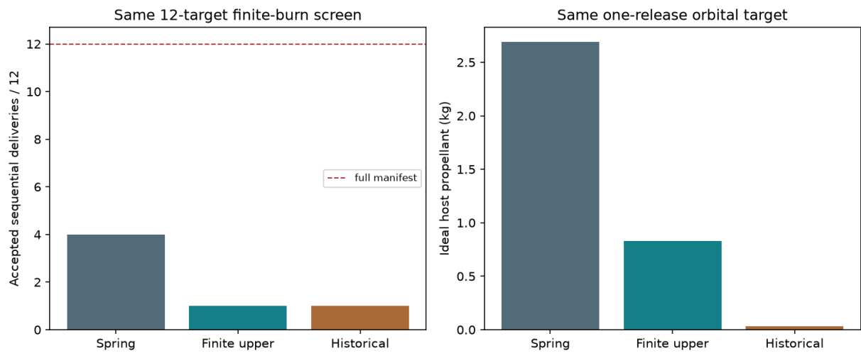
Figure 7: Matched reference results; assumed host and device classes.
