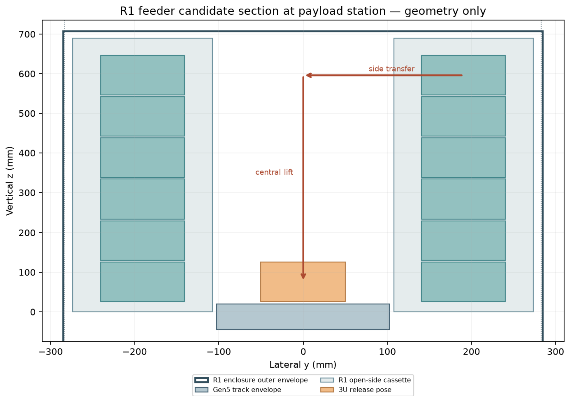
Figure 6: R1 candidate section; geometry drawing, not a qualified mechanism.
