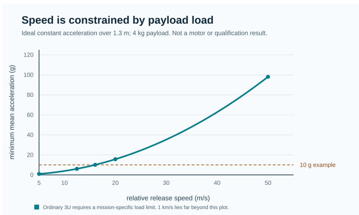
Figure 8: Ideal stroke/load requirements, not a measured VOLLEY command envelope.
