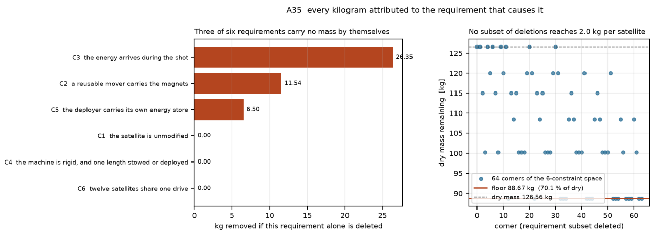
Figure 15: Constraint and mass-attribution analysis; mass is a model rollup.
