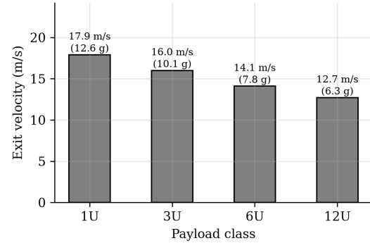
Fig. 17. Payload family: force-limited above 1U; velocity, not safety, is traded. †Counts are volumetric , calibrated so the 3U case returns the twelve the machine is laid out for. A subsequent fixed-cell design study replaces them where a cell geometry actually exists: 1U gives 36 per load at 2.125 kg , not 40 at 1.92, because three 100 mm units plus two dividers leave 37.5 mm of a 340.5 mm cell unusable, and ThinSat and 12U are refused outright because two of their dimensions exceed the 100 mm cell section. The binding constraint is the 166 mm cassette width.
