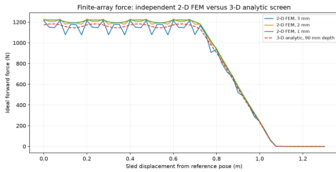
Fig. 22. Finite Gen5 force profiles from a 2-D magnetostatic FEM at three mesh sizes and the 3-D analytic cuboid-field screen. Both use ideal phase. The 2-D solve omits magnet-depth effects; no curve is a measurement.
