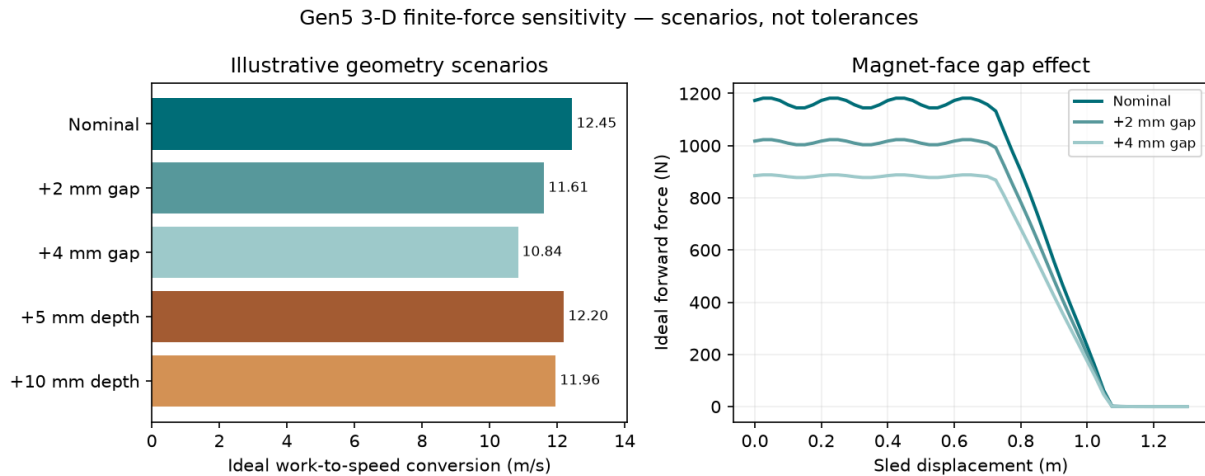
Figure 4: Ideal finite-force gap and depth scenarios; not measured tolerances.
