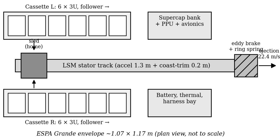
Figure 9: Gen5 layout and mission hardware elements. Diagram from the thesis analysis.
