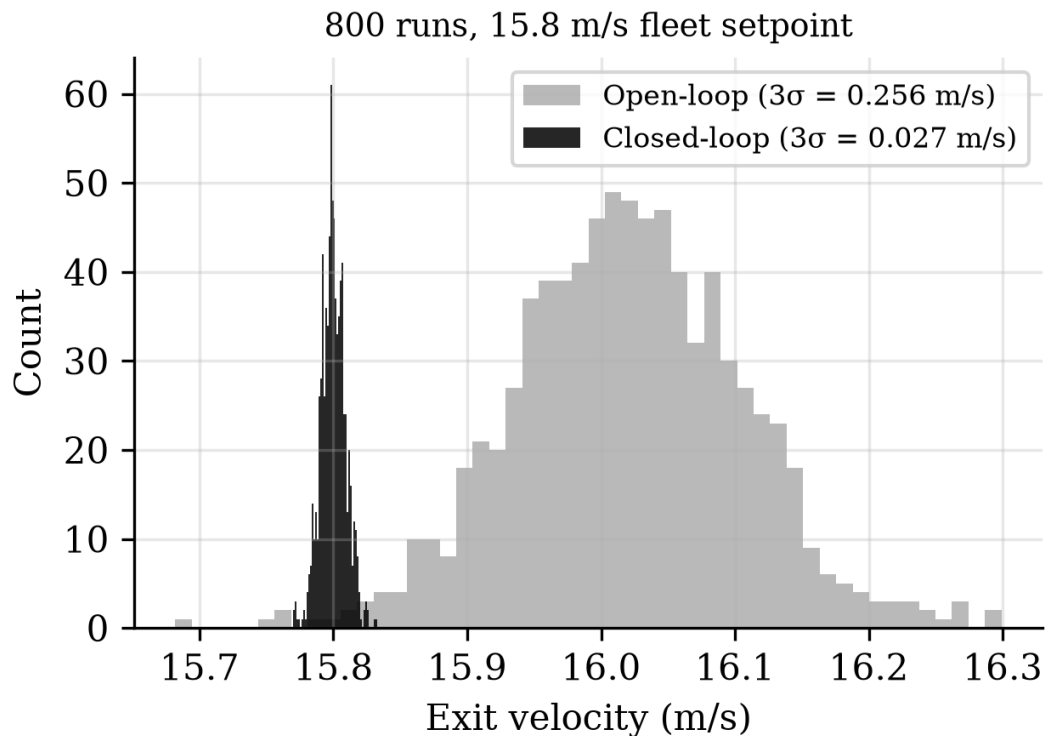
Figure 8: Closed-loop simulation distribution at the fleet setpoint.
