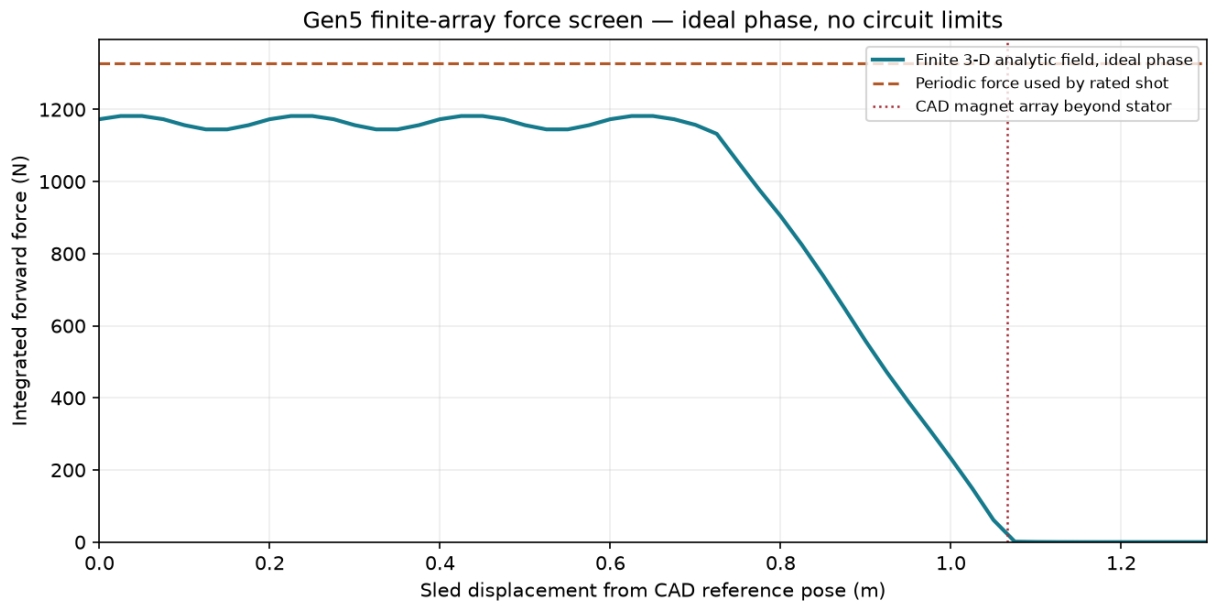
Figure 2: Finite-array/stator model force versus position; no physical measurement.
