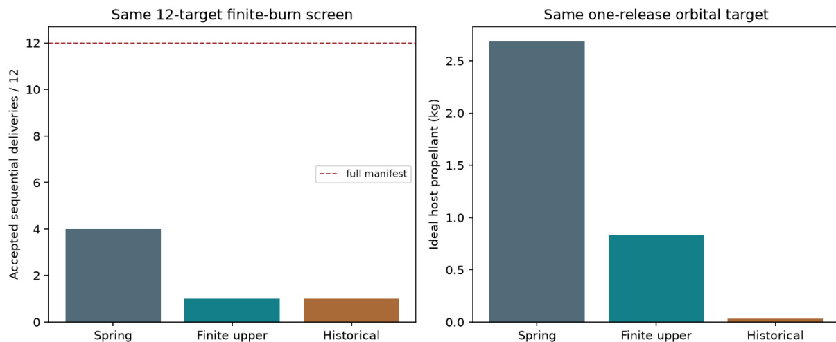
Figure 4: Matched reference results; assumed host and device classes.
