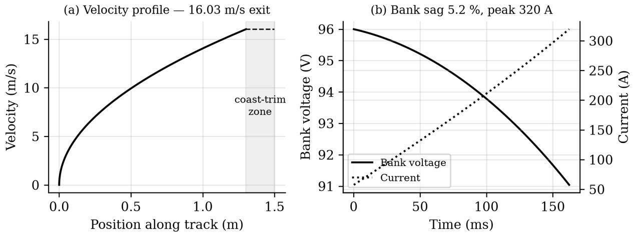
Figure 6: Historical modeled shot: velocity, bank voltage and current.
