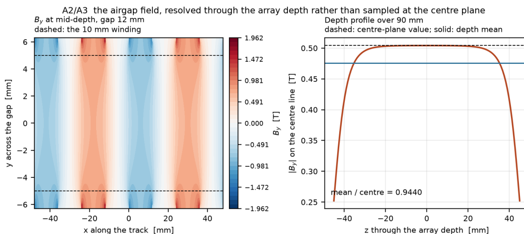
Figure 7: Representative magnetic-field model output. Source: thesis figure A02.
