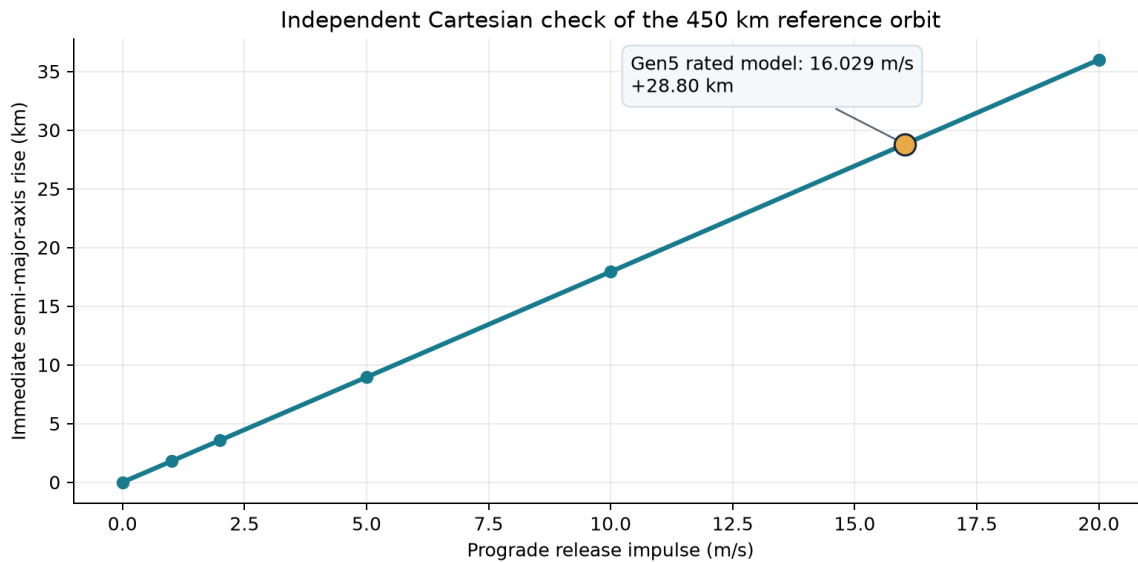
Figure 9: Independent rated-state two-body orbit check. The lifetime claim is outside its scope.
