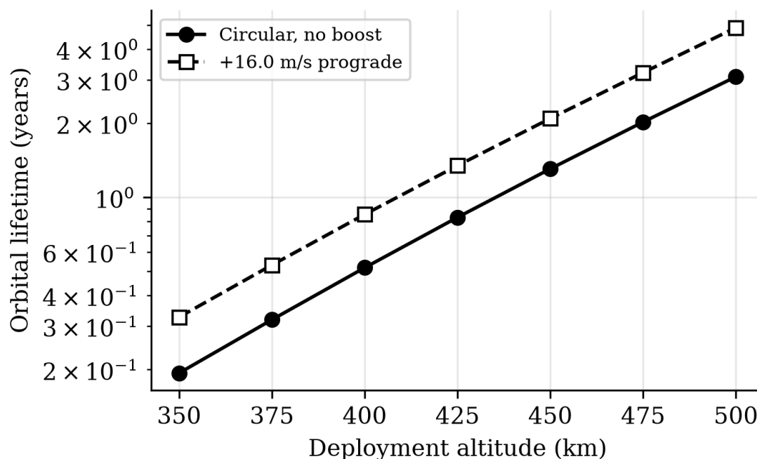
Figure 10: Modelled orbital-lifetime response. Absolute values depend on atmosphere.
