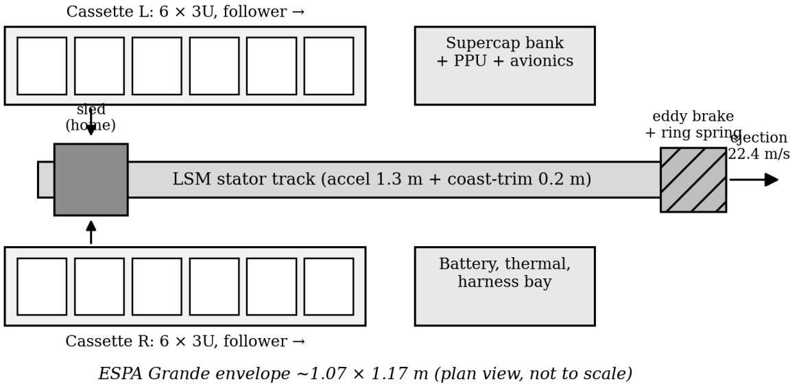
Figure 5: Gen5 layout and mission hardware elements. Diagram from the thesis analysis.
