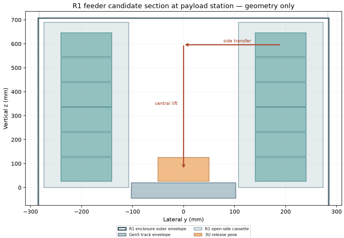
Figure 3: R1 candidate section; geometry drawing, not a qualified mechanism.
