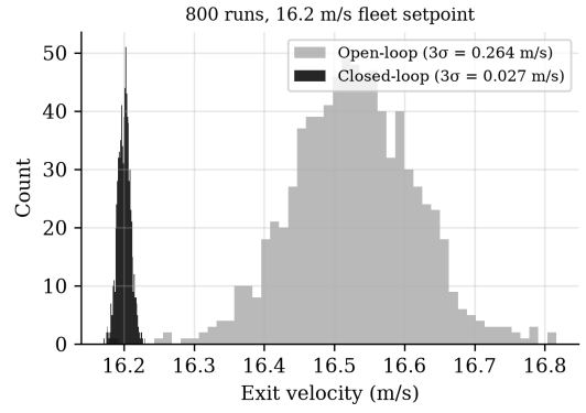
Fig. 6. Closed-loop exit-velocity dispersion, 800 Monte Carlo runs.
