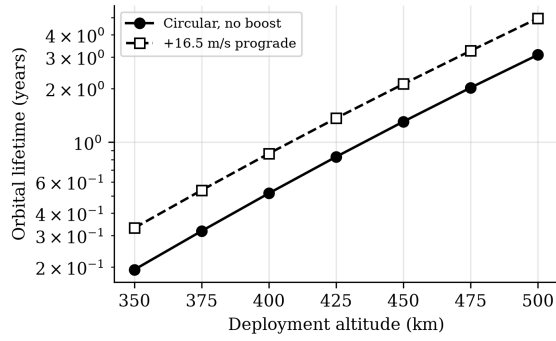
Fig. 7. Orbital lifetime vs deployment altitude (BC = 61 kg/m 2 , mean activity).
