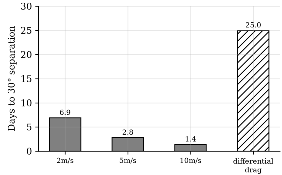
Fig. 13. Constellation seeding: velocity splits versus differential drag under identical assumptions. The figure predates the release-timing baseline and omits it; 30° by timed release costs 468 s at zero \Delta v and would plot at the origin of this axis. It is retained because the drag comparison it makes is still correct, not because the comparison it implies is complete.
