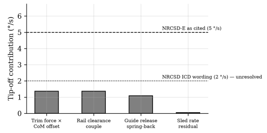
Fig. 15. Tip-off error budget against deployer requirement classes.
