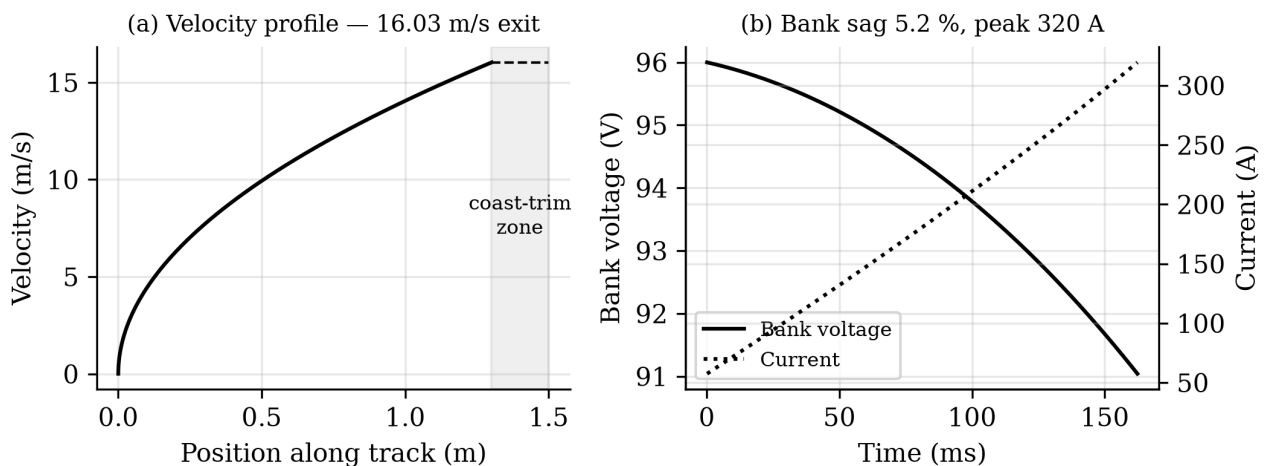
Figure 8: Historical modeled shot: velocity, bank voltage and current.
