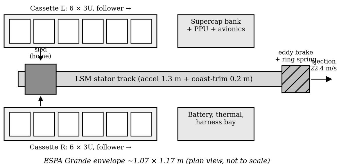
Figure 7: Gen5 layout and mission hardware elements. Diagram from the thesis analysis.
