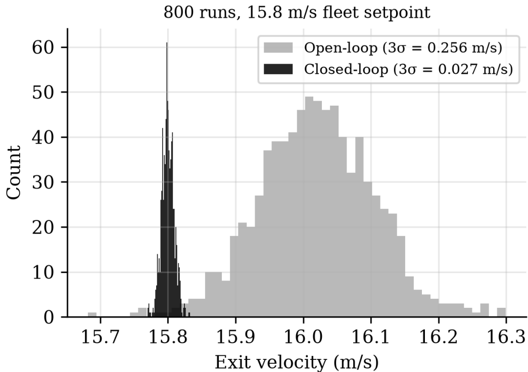
Figure 10: Closed-loop simulation distribution at the fleet setpoint.
