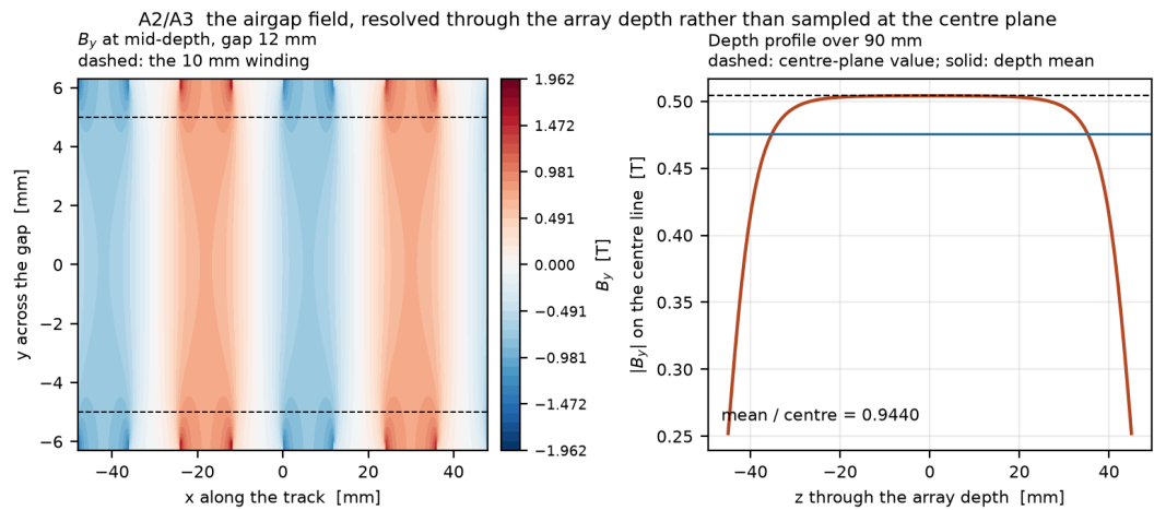
Figure 9: Representative magnetic-field model output. Source: thesis figure A02.
