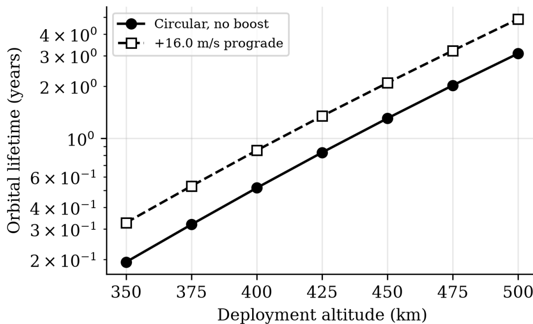
Figure 12: Modelled orbital-lifetime response. Absolute values depend on atmosphere.
