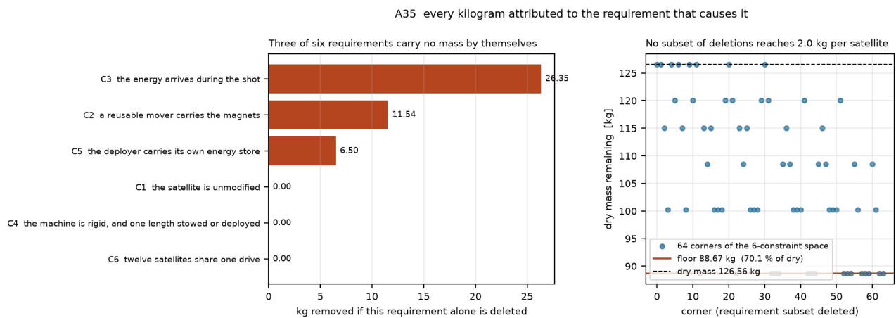
Figure 13: Constraint and mass-attribution analysis; mass is a model rollup.
