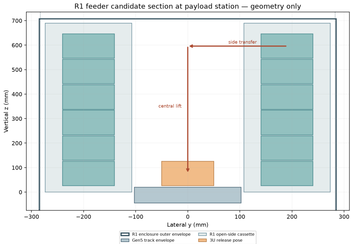
Figure 5: R1 candidate section; geometry drawing, not a qualified mechanism.
