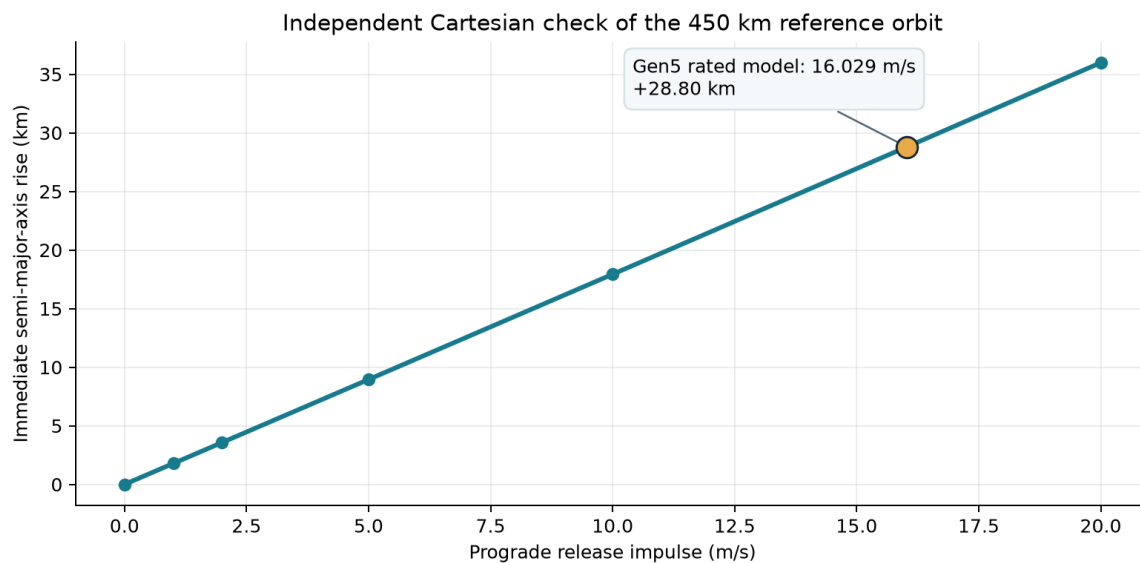
Figure 11: Independent rated-state two-body orbit check. The lifetime claim is outside its scope.
