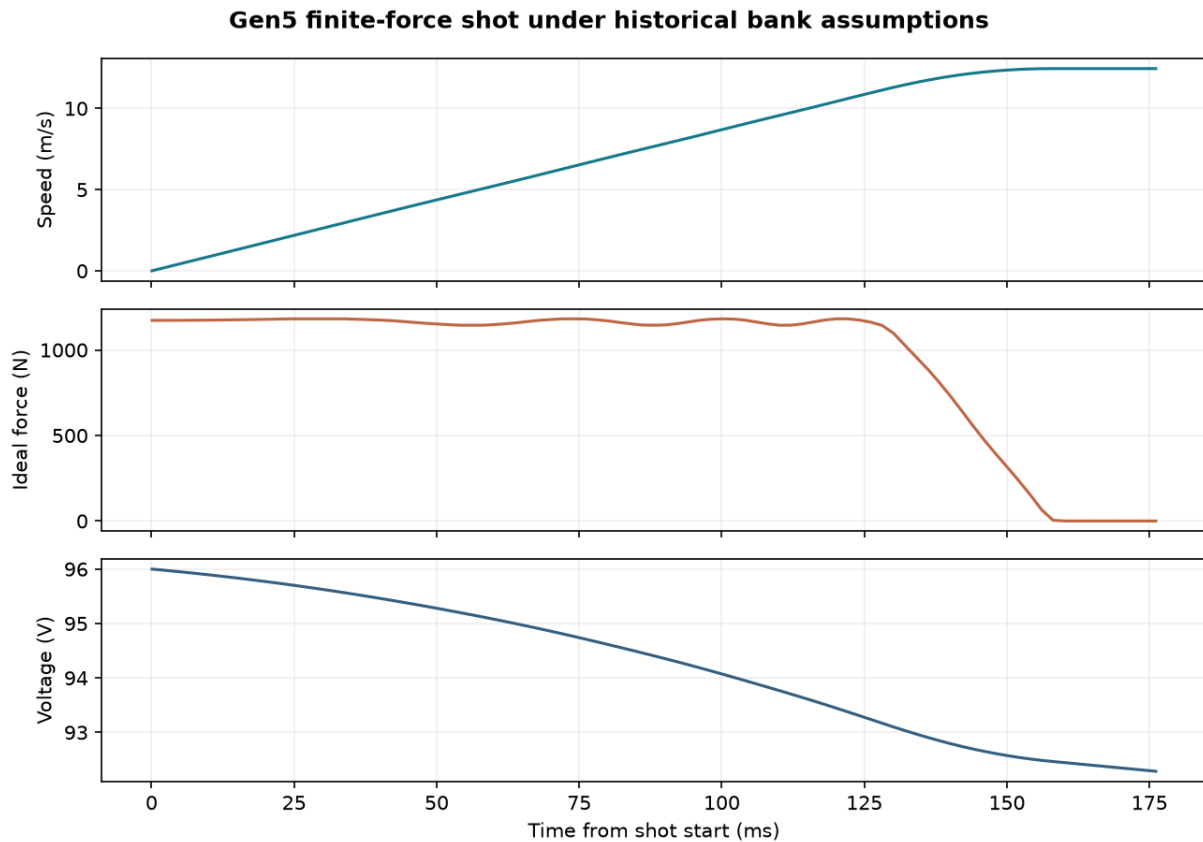
Figure 4: Finite-force speed and assumed bank energy histories.
