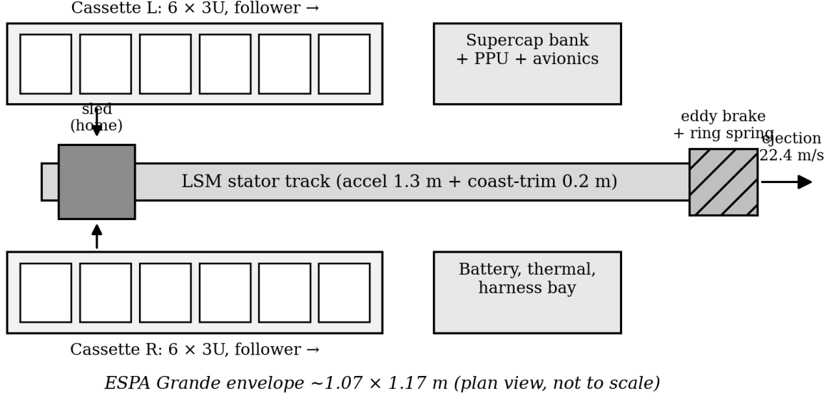
Figure 7: Gen5 layout and mission hardware elements. Diagram from the thesis analysis.
