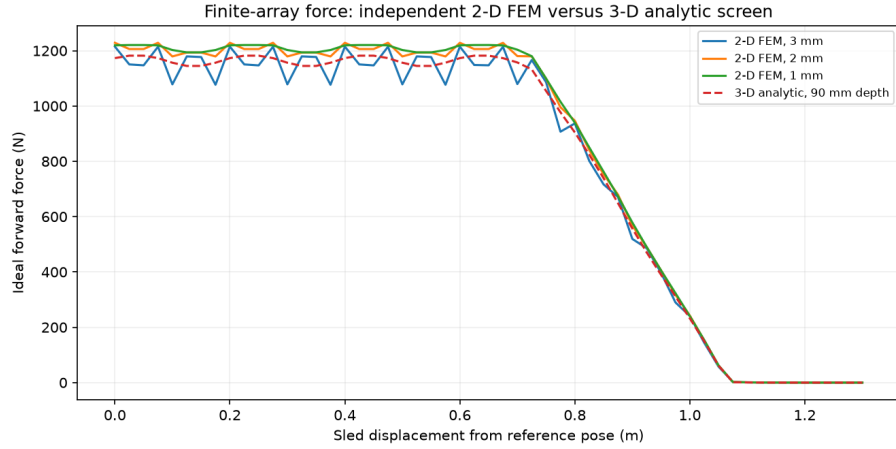
Figure 4: Independent 2-D finite-element force comparison
