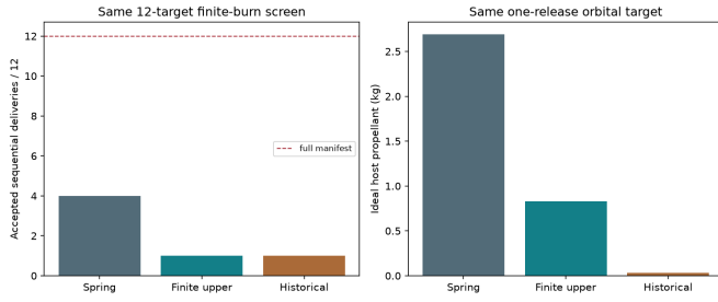
Fig. 23. Matched reference inputs and bounded optimizer outcomes. No sampled twelve-shot option closes; assumed device masses and host performance are not supplier data.
