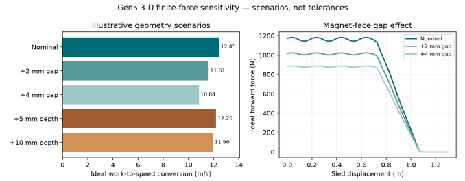
Fig. 22. Deterministic ideal-force scenarios for face gap and depth offset. The 14 mm face gap gives 0.907 kJ versus 1.042 kJ at 12 mm; these are assumed geometry changes, not measured tolerances or achieved speed.
