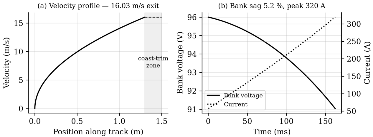
Figure 9: Historical modeled shot: velocity, bank voltage and current.
