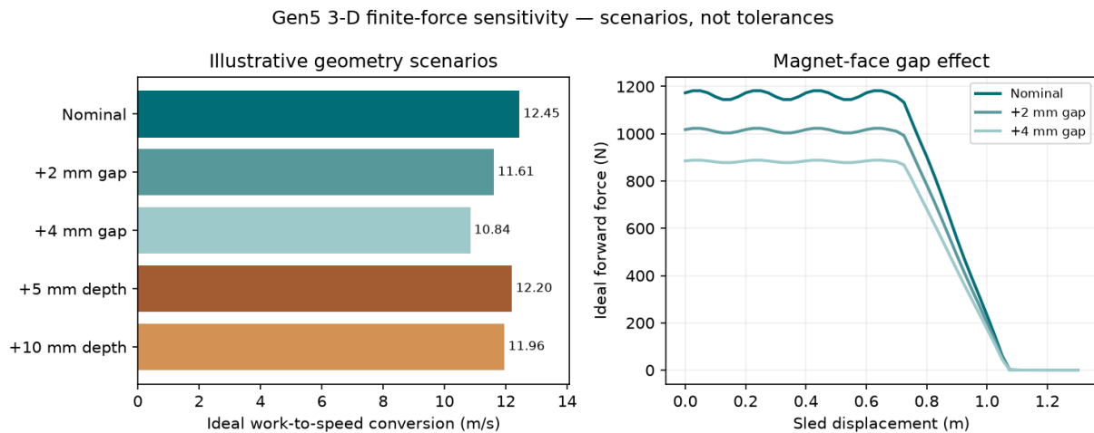
Figure 4: Ideal finite-force gap and depth scenarios; not measured tolerances.
