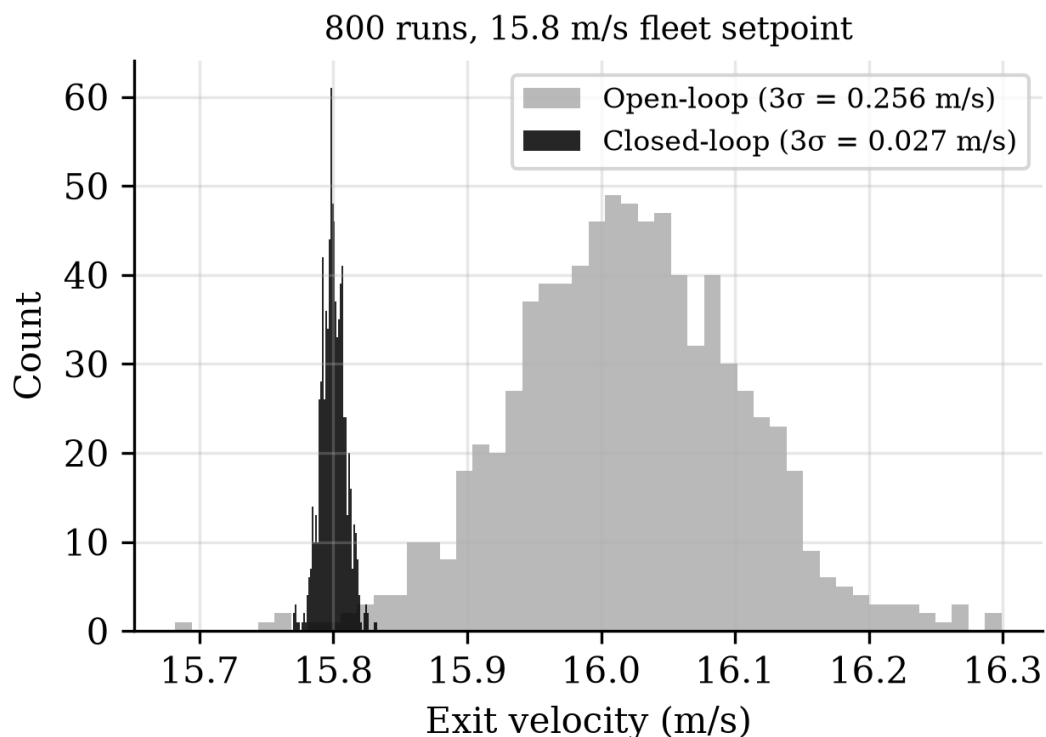
Figure 11: Closed-loop simulation distribution at the fleet setpoint.
