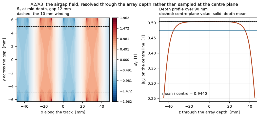
Figure 10: Representative magnetic-field model output. Source: thesis figure A02.
