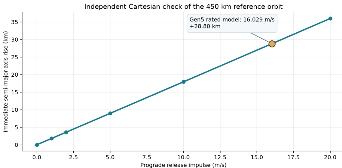
Figure 12: Independent rated-state two-body orbit check. The lifetime claim is outside its scope.
