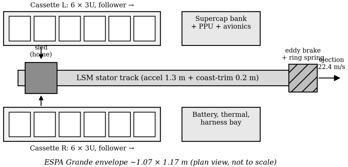
Figure 8: Gen5 layout and mission hardware elements. Diagram from the thesis analysis.
