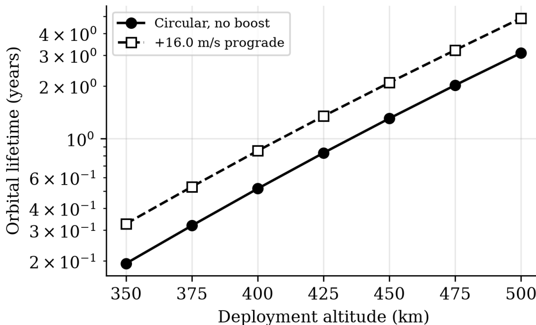
Figure 13: Modelled orbital-lifetime response. Absolute values depend on atmosphere.
