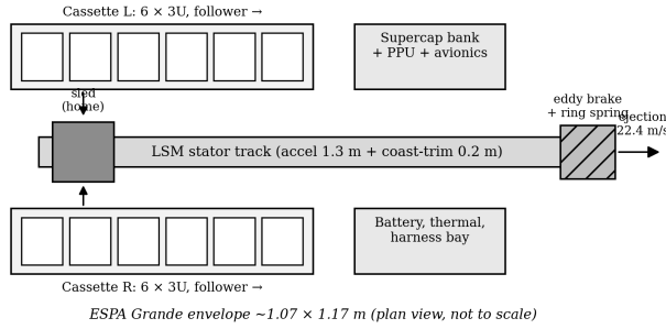
Fig. 2. Plan-view layout against an ESPA-Grande-class envelope (not to scale). The closed envelope currently exceeds that class in length; see Sec. XV.
