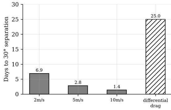
Fig. 9. Constellation seeding: EMOC velocity splits versus differential drag under identical assumptions.
