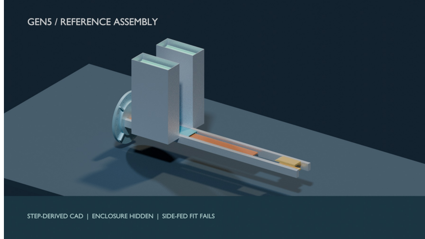
Figure 1: STEP-derived Gen5 reference assembly, enclosure hidden; reference placement has a known track/cassette clash.
