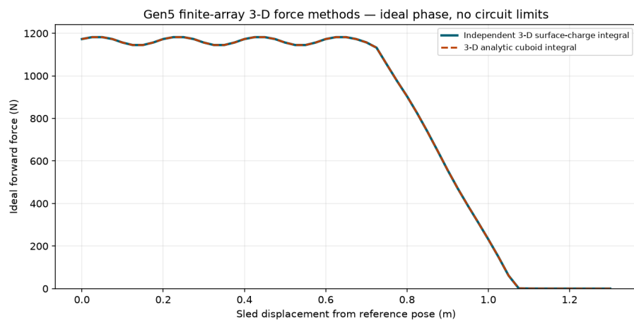
Figure 3: Independent depth-resolved force cross-check
