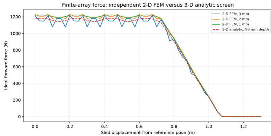
Figure 5: Independent 2-D finite-element force comparison
