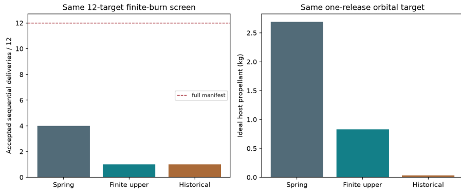
Figure 7: Matched reference mission
