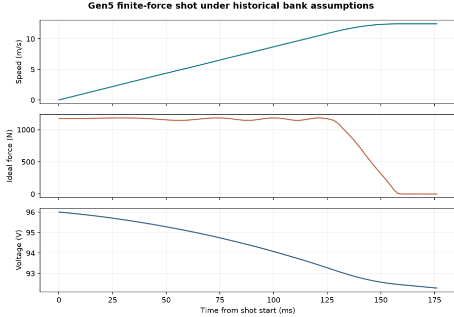
Figure 6: Conditional finite-force shot histories
