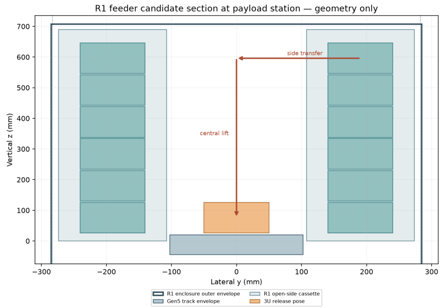
Figure 8: Unselected R1 geometry section
