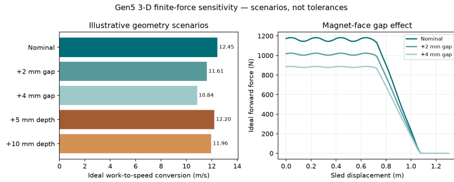
Figure 4: Ideal finite-force geometry sensitivity
