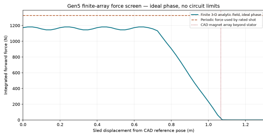
Figure 2: Finite analytic force map
