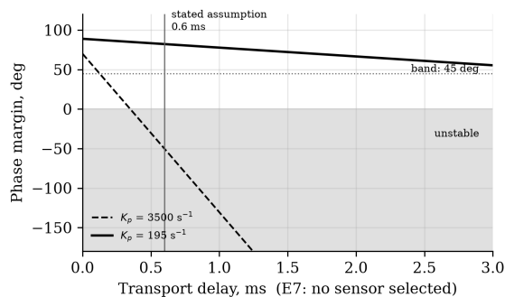
Fig. 8. Phase margin against transport delay. The earlier gain crosses into instability at 0.35 ms of transport delay; the designed gain holds more than 55° across the whole swept range.
