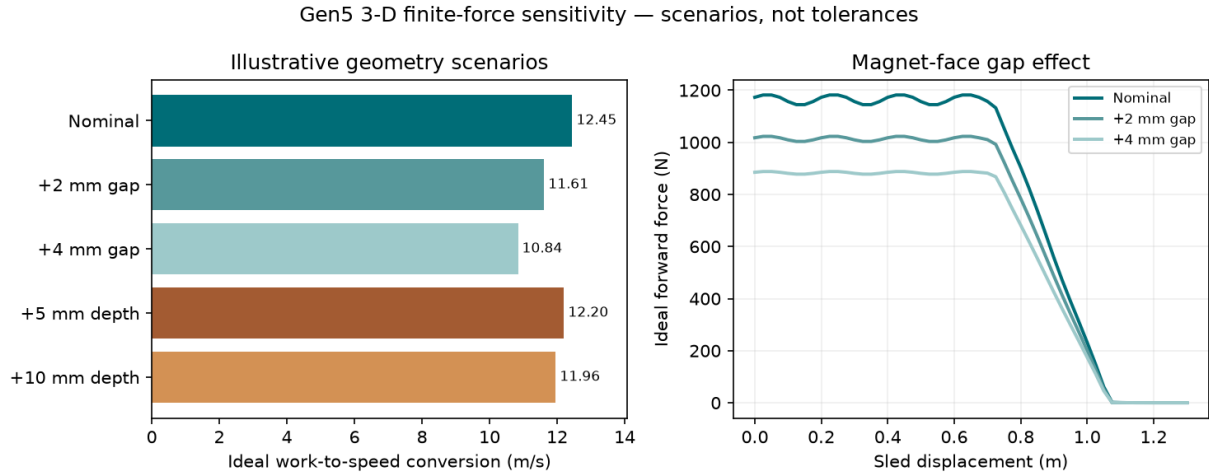
Figure 4: Ideal gap/depth sensitivity; scenarios rather than measured tolerances.
