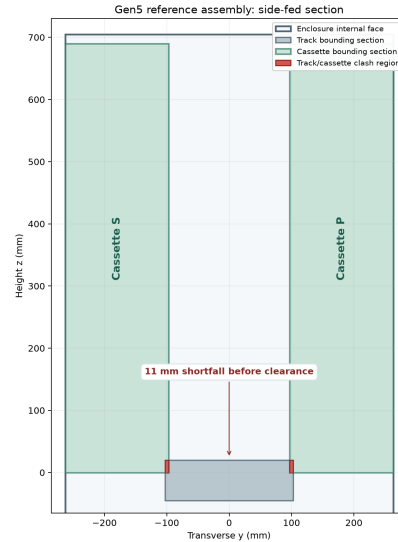
Figure 4. Dimension-derived cross-section and exact-solid clash. Reference placement, not a production drawing.
