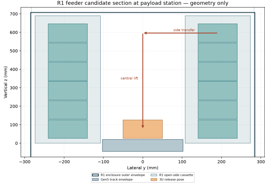
Figure 3: Unselected R1 geometry section
