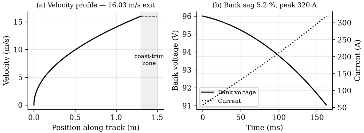
Figure 6: Modelled shot: velocity, bank voltage and current at the rated point.
