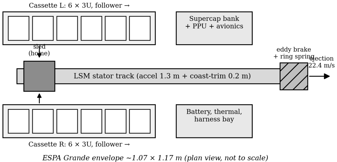
Figure 5: Gen5 layout and mission hardware elements. Diagram from the thesis analysis.
