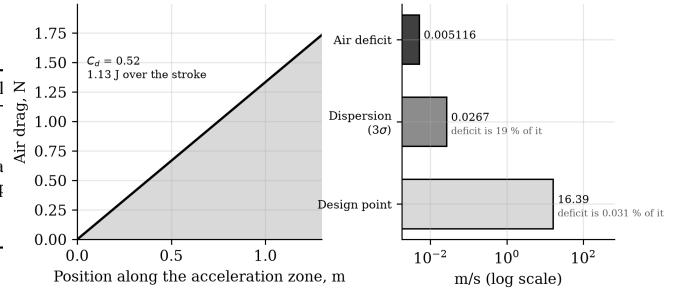
Fig. 15. Air drag along the acceleration zone, and the resulting exit-velocity deficit set against the design point and against the dispersion a ground test exists to resolve.
