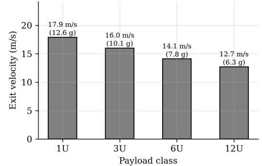
Fig. 14. Payload family: force-limited above 1U; velocity, not safety, is traded. †Counts are volumetric , calibrated so the 3U case returns the twelve the machine is laid out for. A subsequent fixed-cell design study replaces them where a cell geometry actually exists: 1U gives 36 per load at 2.125 kg , not 40 at 1.92, because three 100 mm units plus two dividers leave 37.5 mm of a 340.5 mm cell unusable, and ThinSat and 12U are refused outright because two of their dimensions exceed the 100 mm cell section. The binding constraint is the 166 mm cassette width.
