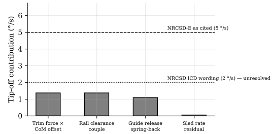
Fig. 13. Tip-off error budget against deployer requirement classes.
