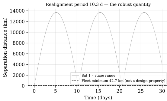
Fig. 12. Satellite-stage range over 30 days, staggered firing at the rated velocity.
