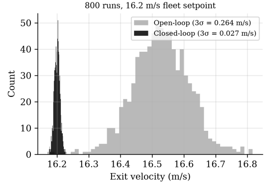
Fig. 6. Closed-loop exit-velocity dispersion, 800 Monte Carlo runs.
