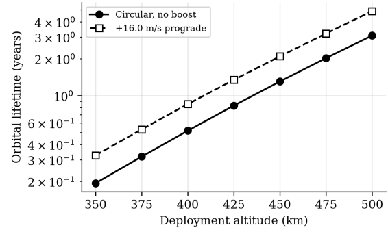
Fig. 9. Orbital lifetime vs deployment altitude (BC = 61 kg/m 2 , mean activity).
