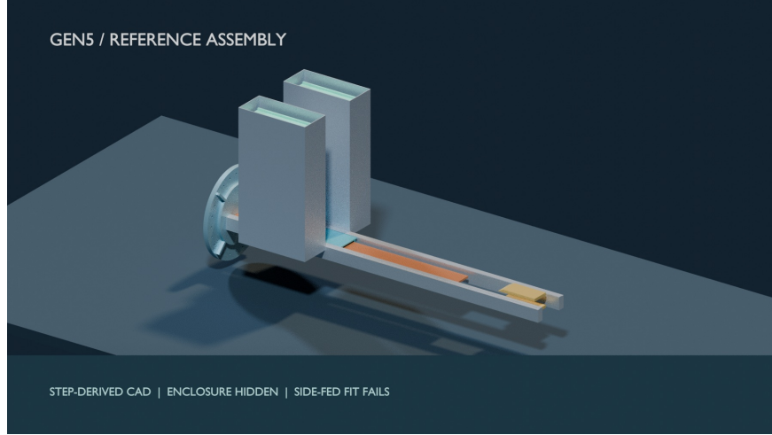
Figure 1: STEP-derived Gen5 reference assembly, enclosure hidden; reference placement has a known track/cassette clash.
