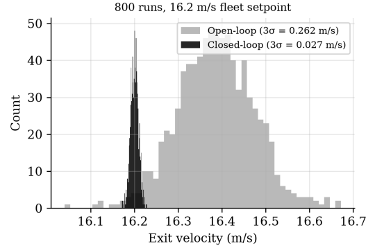
Fig. 8. Closed-loop exit-velocity dispersion, 800 Monte Carlo runs.
