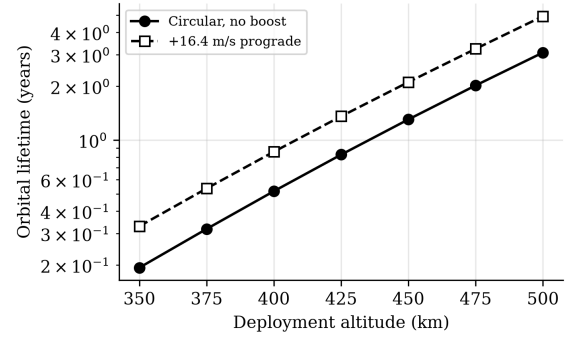
Fig. 7. Orbital lifetime vs deployment altitude (BC = 61 \text{ kg/m}^2 , mean activity).
