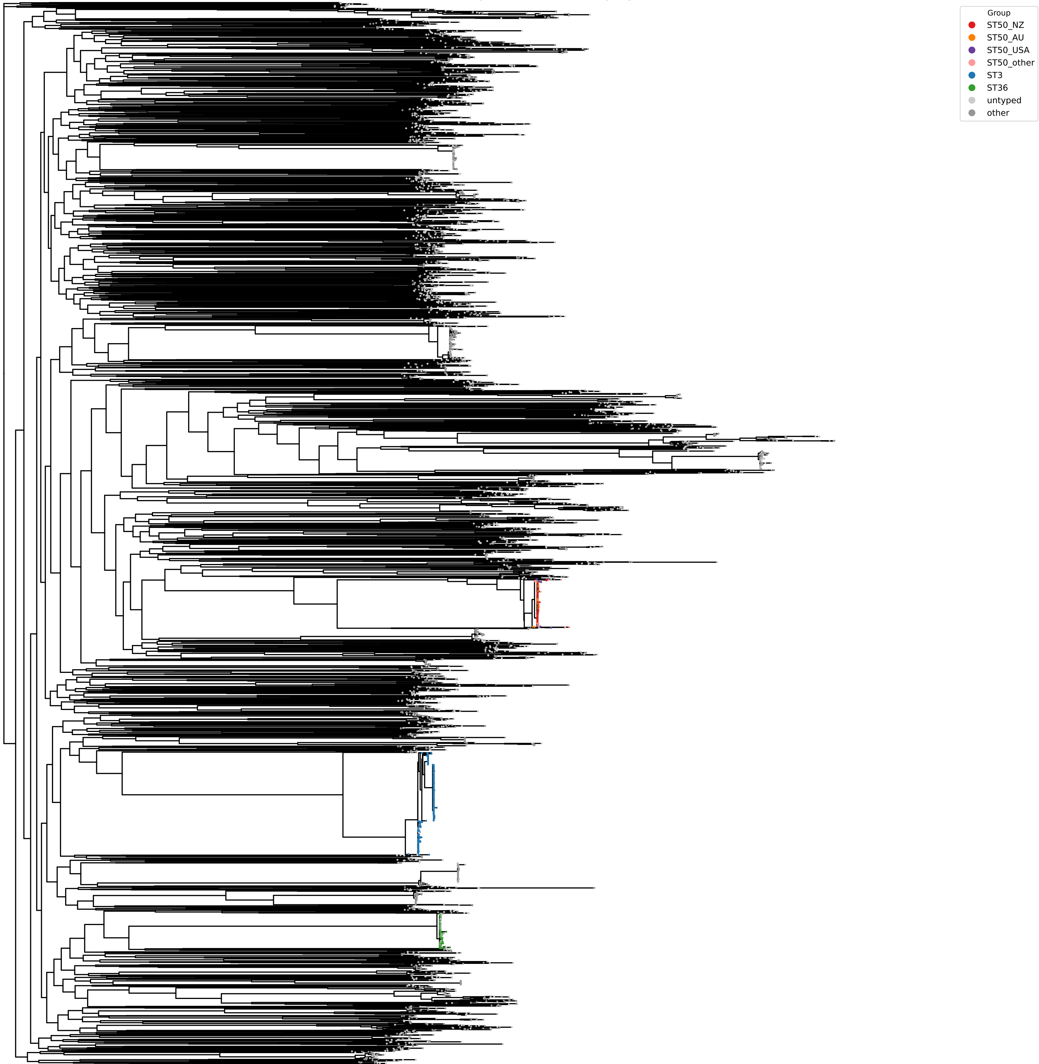
Global VP tree (5,225 genomes) — ST50 highlighted
