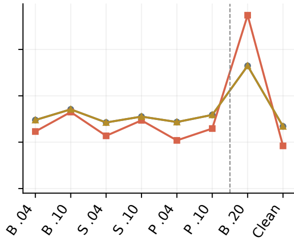
Fashion masks
