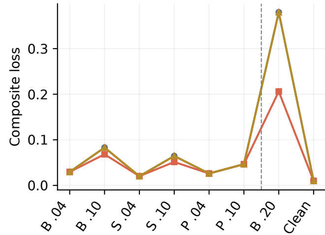
Shapes
