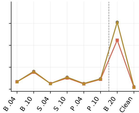
MNIST masks
