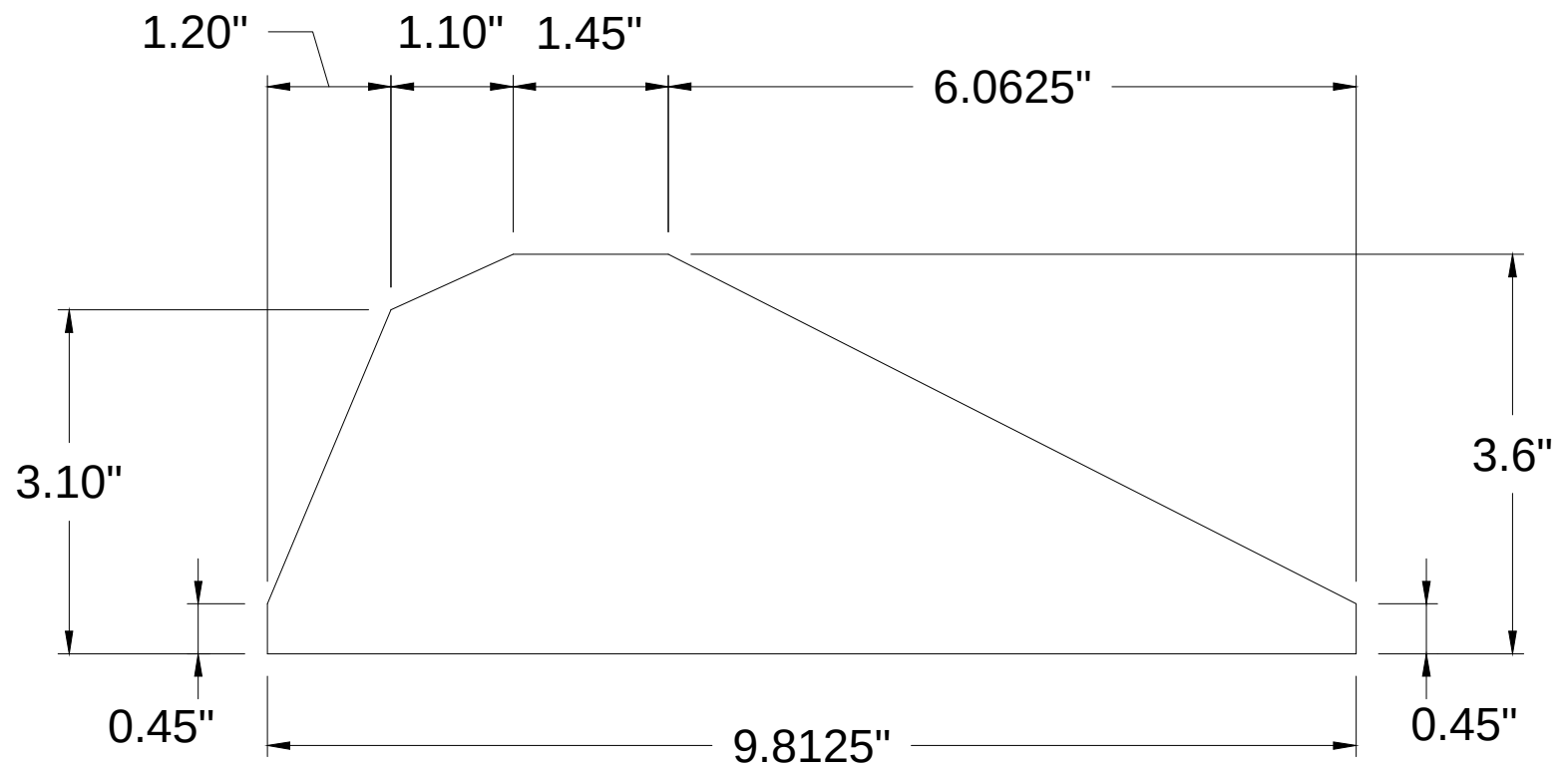
Approx. Fin Dimension for 3" Punisher
