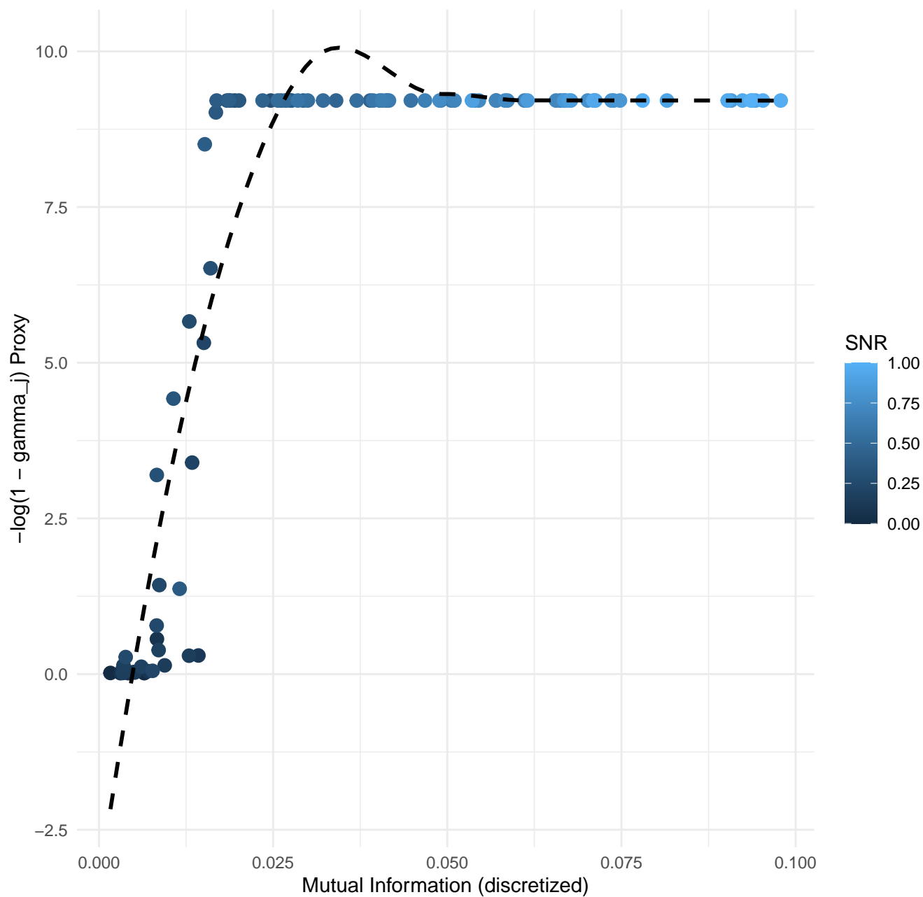
Validation of Proposition 4: Proxy vs True MI
