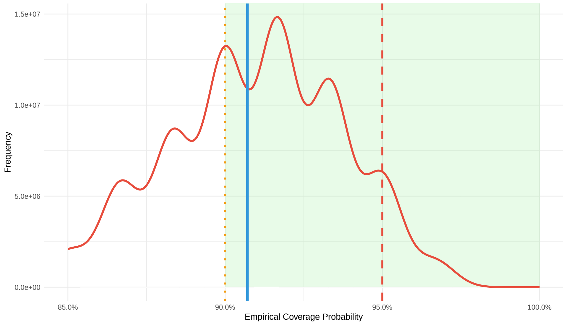
Simulation Validation: ACI Coverage Across 1,000 Synthetic Scenarios
