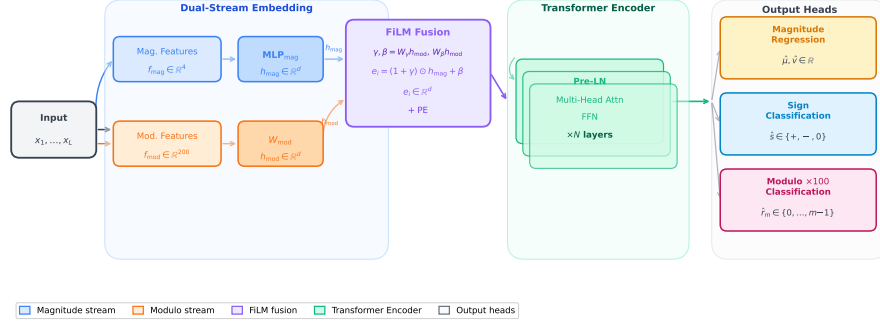
Fig. 1. IntSeqBERT architecture. The Dual-Stream Embedding block projects \mathbf{f}^{\text{mag}} \in \mathbb{R}^4 and \mathbf{f}^{\text{mod}} \in \mathbb{R}^{200} each to \mathbb{R}^d and fuses them via FiLM. Positional encodings are added to the fused embedding before the Pre-LN Transformer encoder, which outputs to three prediction heads (magnitude regression, sign classification, 100 \times Modulo classification).
