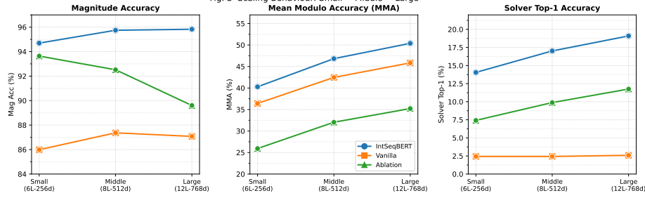
Fig. 7. Scaling behaviour across model sizes (Small / Middle / Large). Left: Magnitude accuracy (Mag Acc) remains high for both IntSeqBERT and Ablation, with only +1.1 pt improvement from Small to Large. Centre: MMA (Mean Modulo Accuracy) for IntSeqBERT improves from 40.3% (Small) to 50.4% (Large, +10.1 pt), consistently exceeding Ablation at all scales. Right: Solver Top-1 accuracy for IntSeqBERT improves from 14.1% to 19.1% (+5.0 pt), with a growing gap over Vanilla ( \approx 2.4\% , flat).
