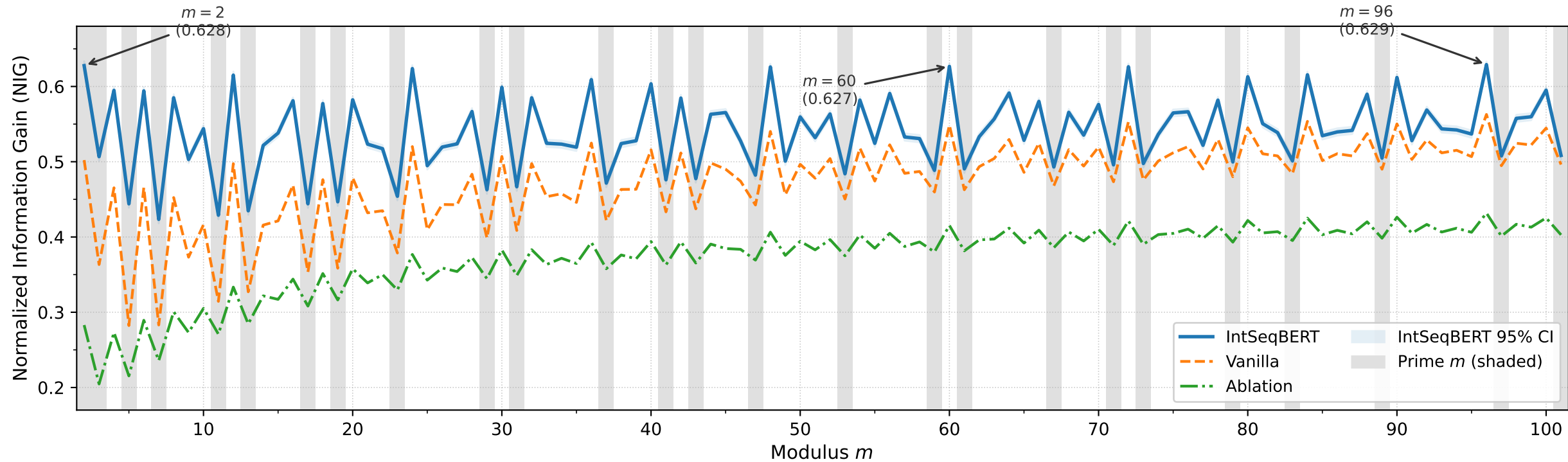
Fig. 2 NIG Spectrum over Moduli m = 2, \dots, 101 (Large models)
