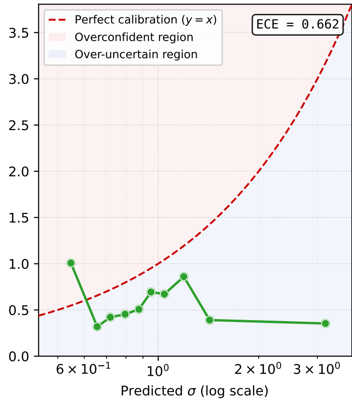
Ablation
