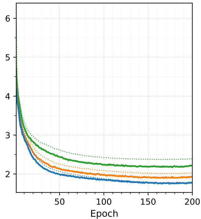
Fig. 4b Train vs. Validation Loss (solid = Val, dotted = Train)
