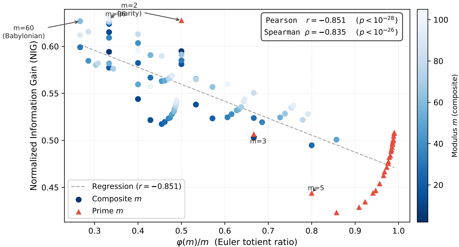
Fig. 2b NIG vs. Euler totient ratio \phi(m)/m (Large IntSeqBERT)
